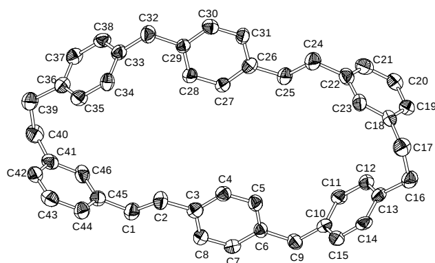
Fig. 3 Crystal-structure analysis of 3
