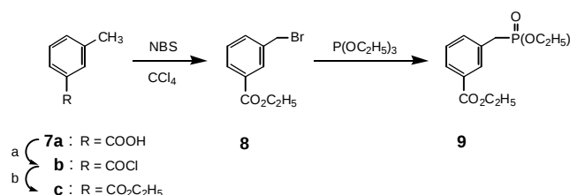
Scheme 1 Preparation of intermediates a: SOCl_2 ; b: C_2H_5OH
